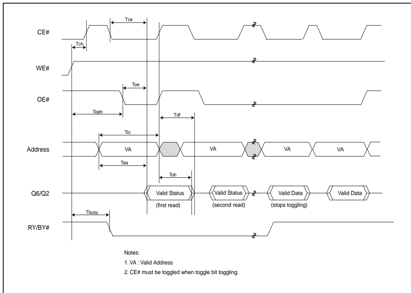
Figure 23. TOGGLE BIT TIMING WAVEFORMS (DURING AUTOMATIC ALGORITHMS)
