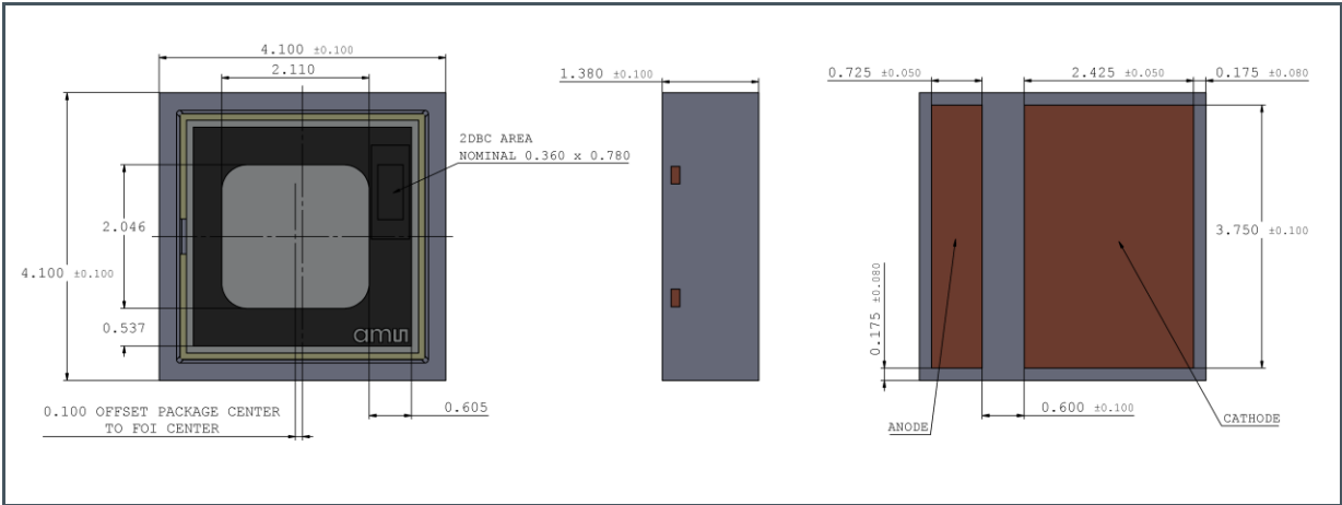
Figure 10: Package Dimensions (1)
