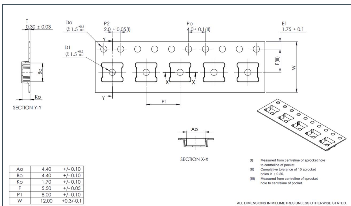
Figure 16: Carrier Tape Dimensions and Overview (1)(2)(3)
