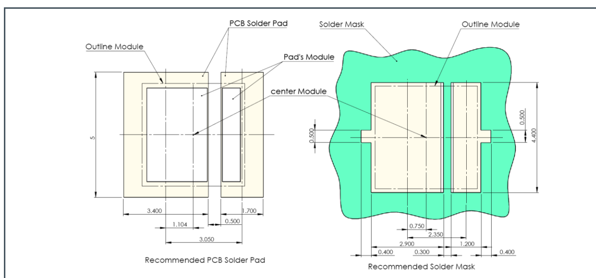
Figure 12: Recommended PCB Pad Layout (top view) (1)
