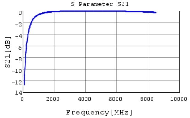
GJM1555C1H3R8BB01 S21 DCOV, 25degC
