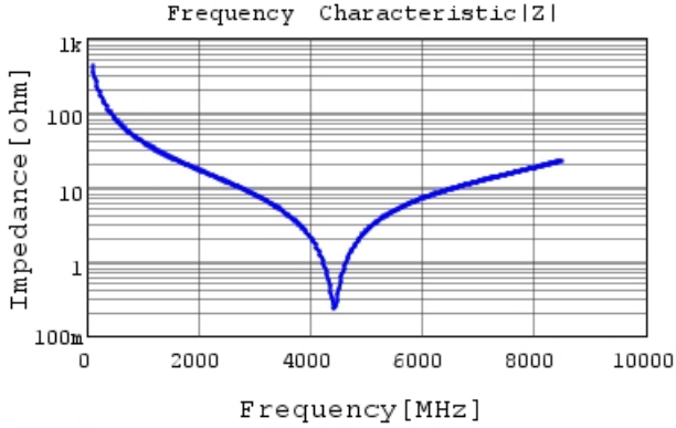
GJM1555C1H3R8BB01 |Z| DCOV, 25degC
