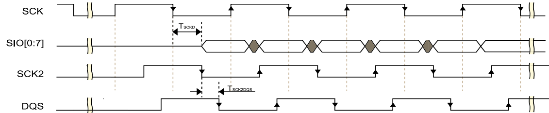
Figure 19. FlexSPI input timing in DDR mode where FlexSPI n _MCR0[RXCLKSRC] = 0x3 (caseB2)
