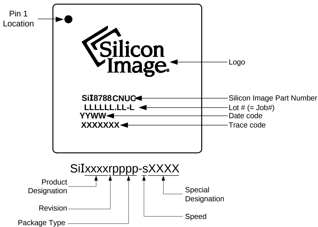
Figure 9.1. Marking Diagram
