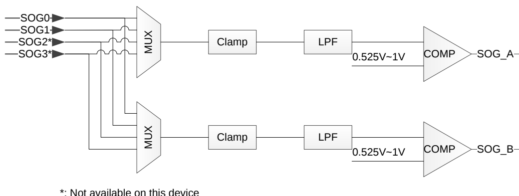
Figure 3.3. Sync Slicers
