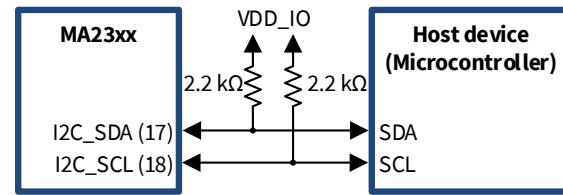
Figure 11.19: I2C serial control interface block diagram
