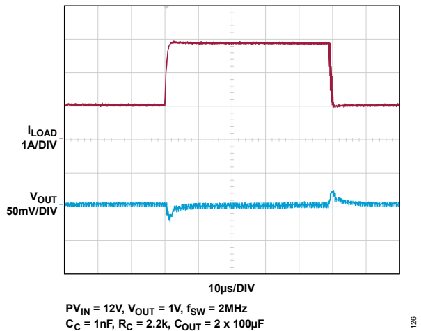
Figure 44. Transient Response: Load Current Stepped from 1A to 3A
