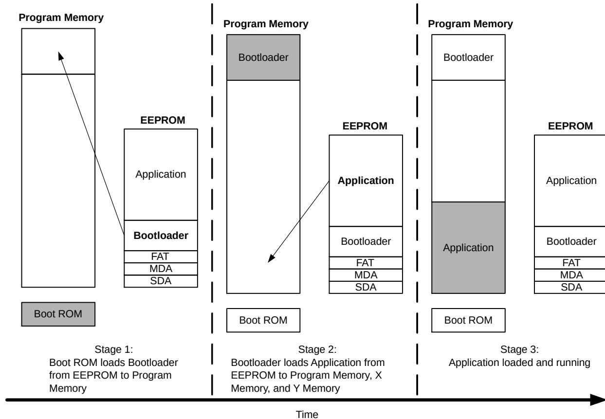
Figure 9. Booting Sequence
