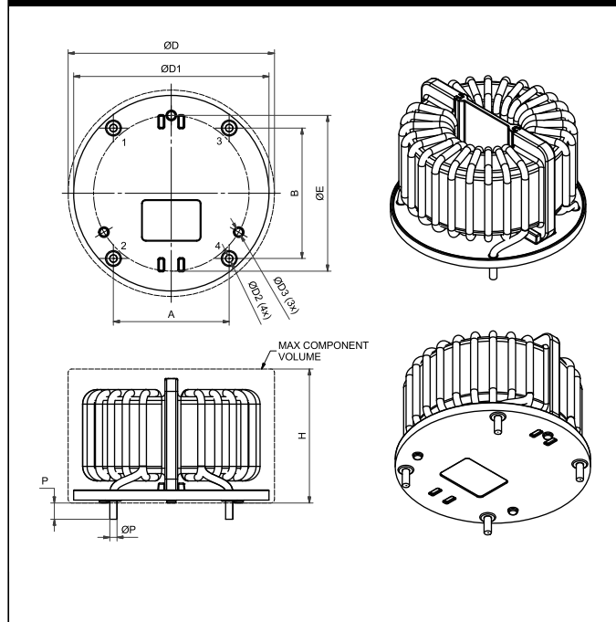
Horizontal 2-line chokes (Size 1-3)
