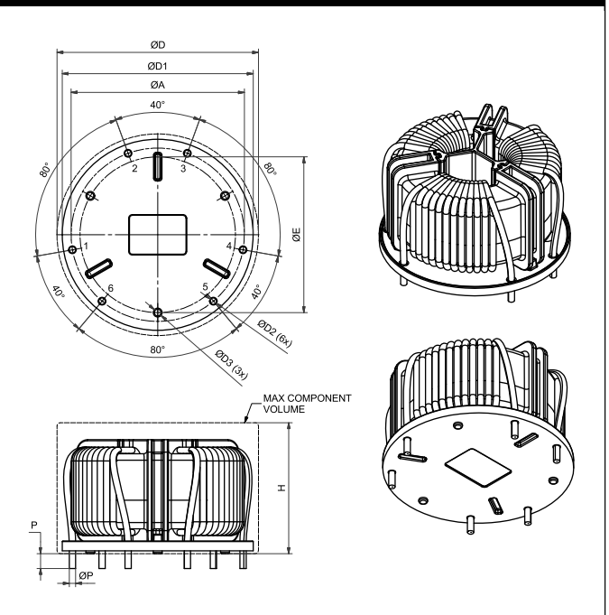
Horizontal 3-line chokes (Size 7-9)
