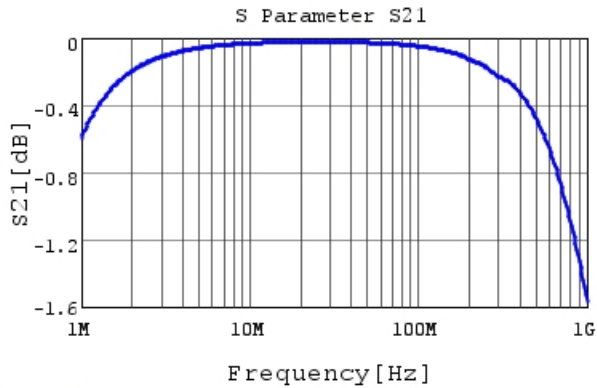
DE2E3SA472MA3BT02F S21 DC0V, 20degC
