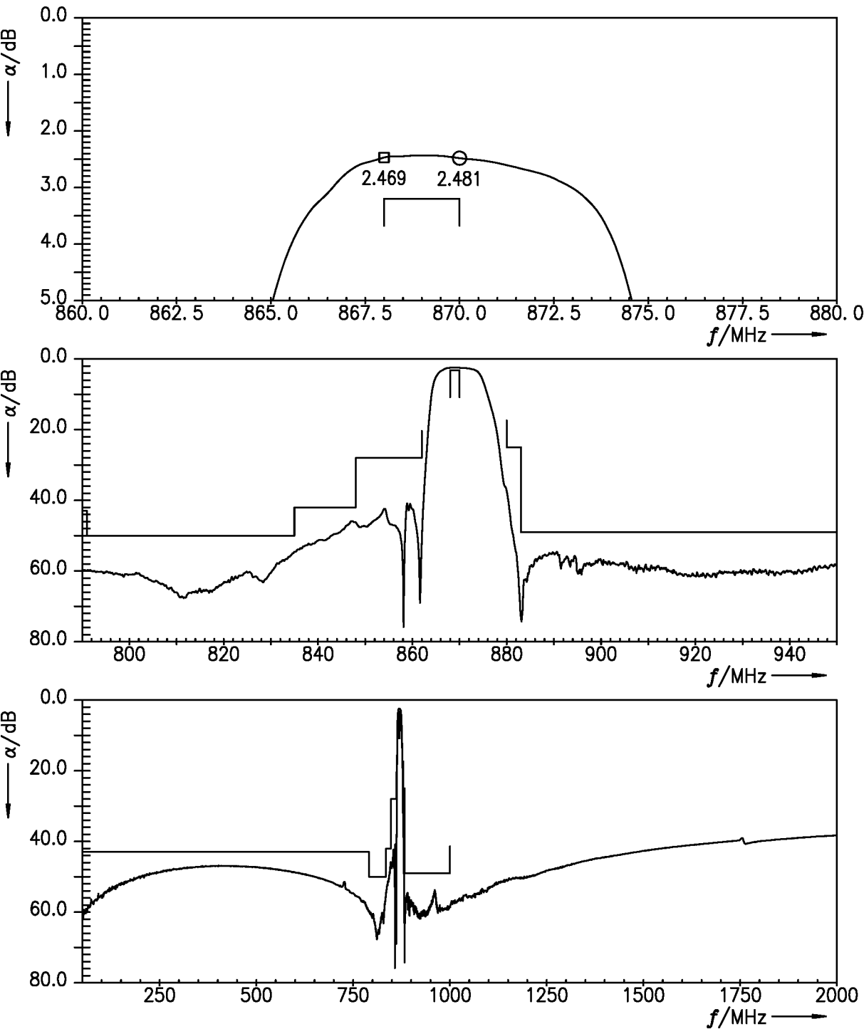
Figure 3: Attenuation.
