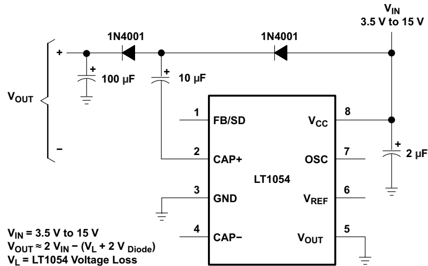
Figure 20. Positive-Voltage Doubler
