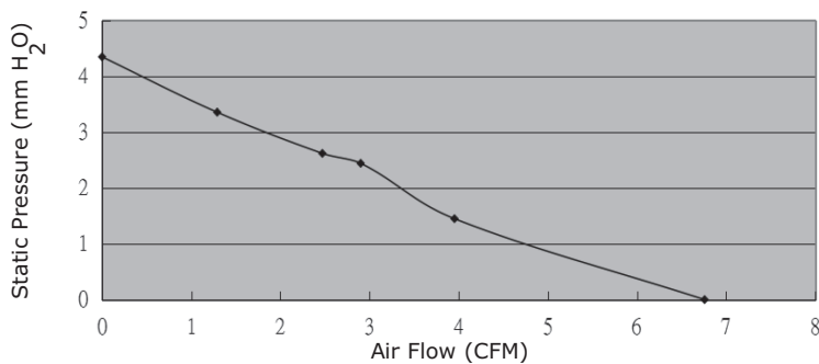
CFM-4010B-180-296
