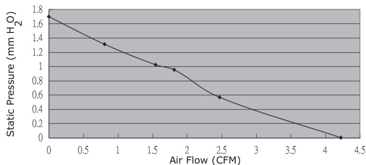
CFM-4010B-050-195
