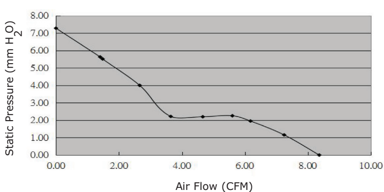
CFM-4015B-175-287
