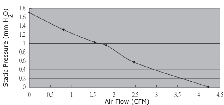
CFM-4010B-150-195
