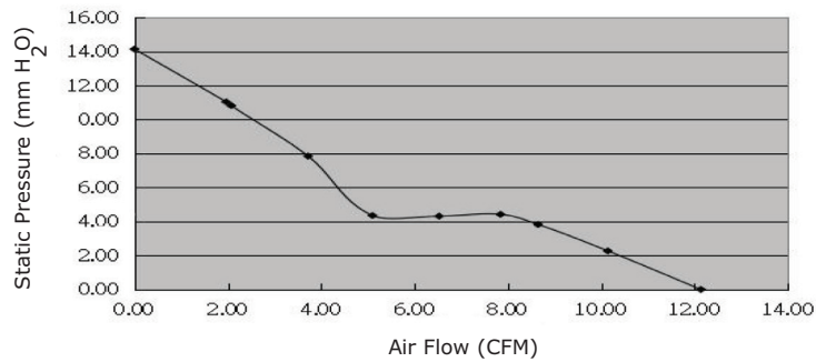
CFM-4015B-1105-365
