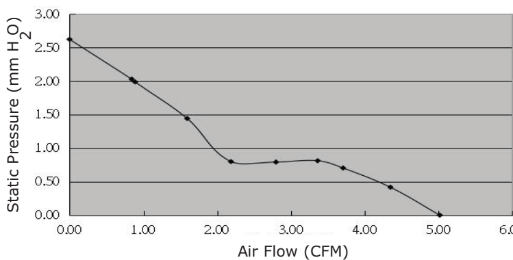
CFM-4015B-145-176
