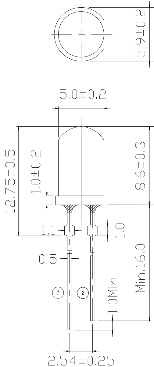
Stopper type
