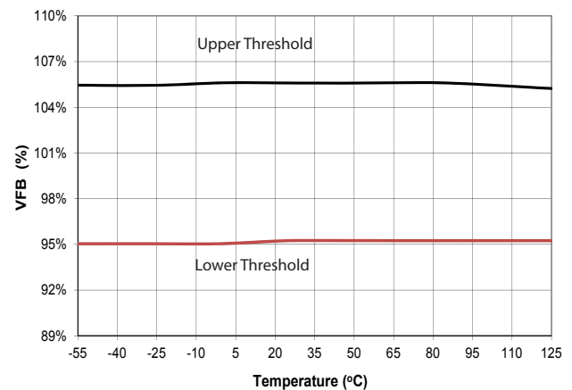
PG Threshold
