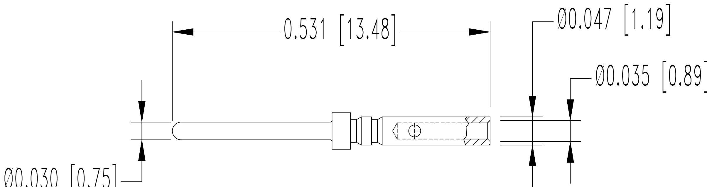
MALE CONTACT 15X (ENLARGED)
