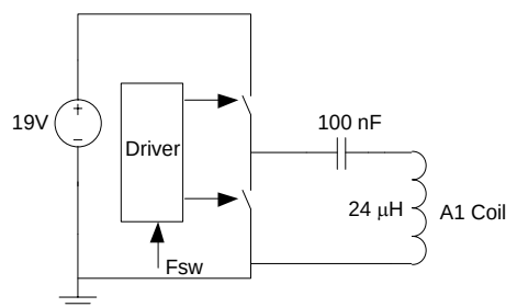
Figure 8. Half Bridge inverter TX Coil Driver.
