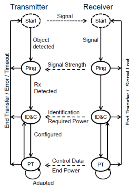
Figure 12. System state machine diagram
