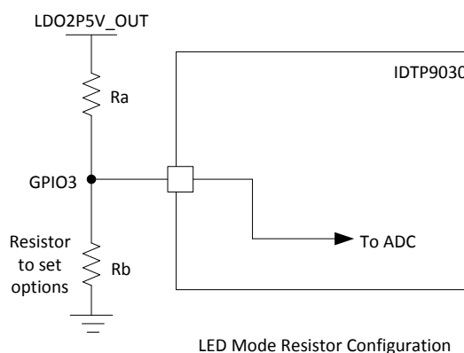
Figure 16. IDTP9030 LED Resistor Options.
