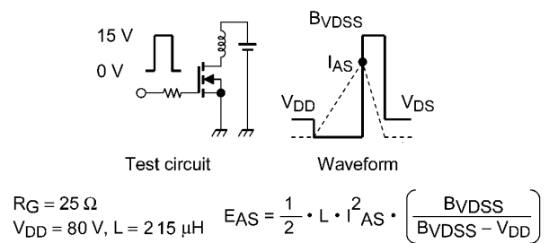
Fig. 8.15 Test Circuit/Waveform
