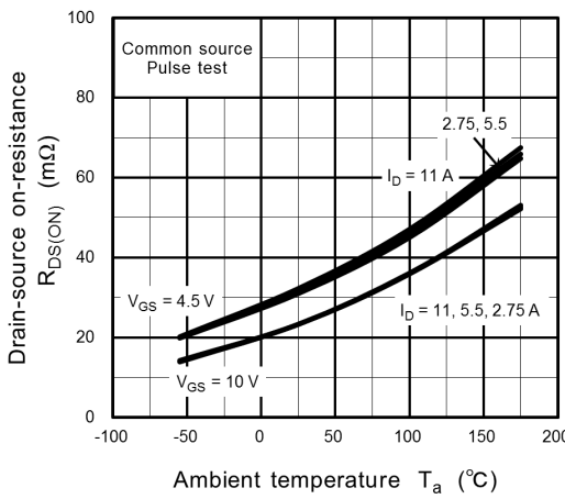
Fig. 8.6 R_{DS(ON)} - T_a
