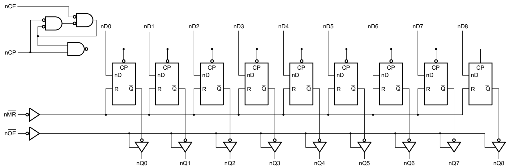
Fig. 4. Logic diagram
