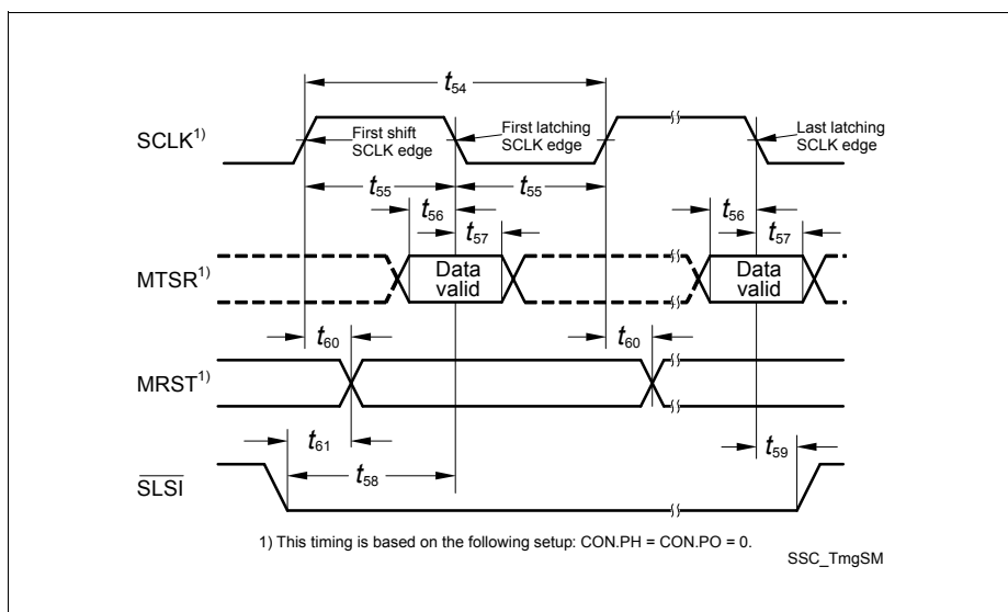
Figure 35 SSC Slave Mode Timing
