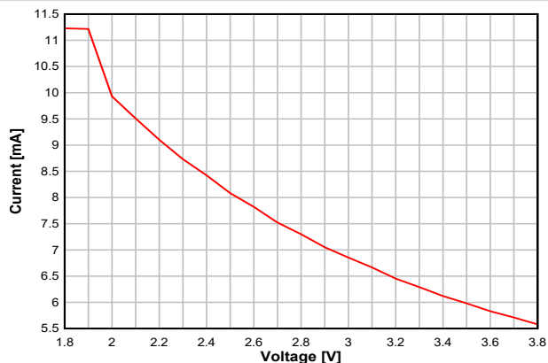
Figure 8-7. RX Current vs. Supply Voltage (VDD) (BLE 1 Mbps, 2.44 GHz)
