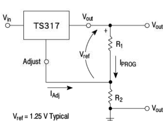
Figure 17. Basic Circuit Configuration
