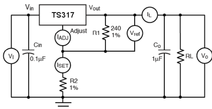
Figure 3. Standard Test Circuit
