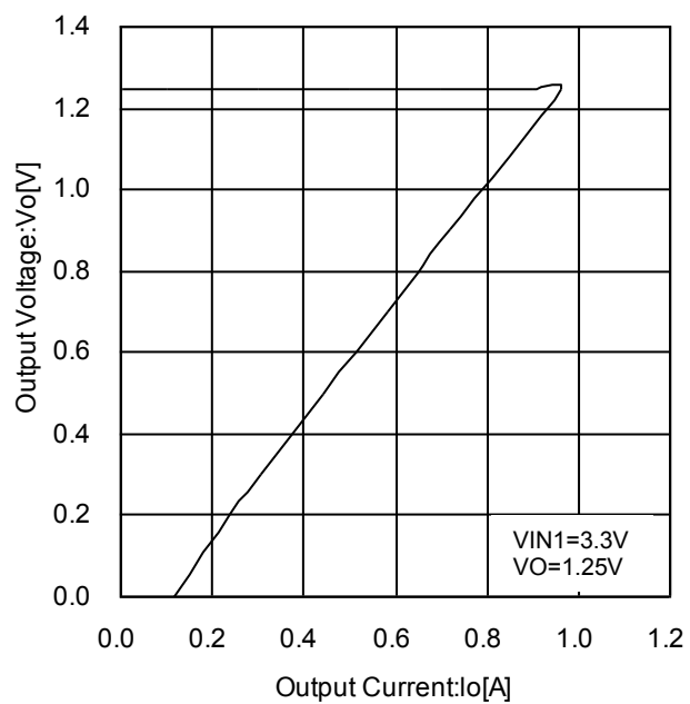
Figure 30. REG1 Output Voltage vs Output Current
