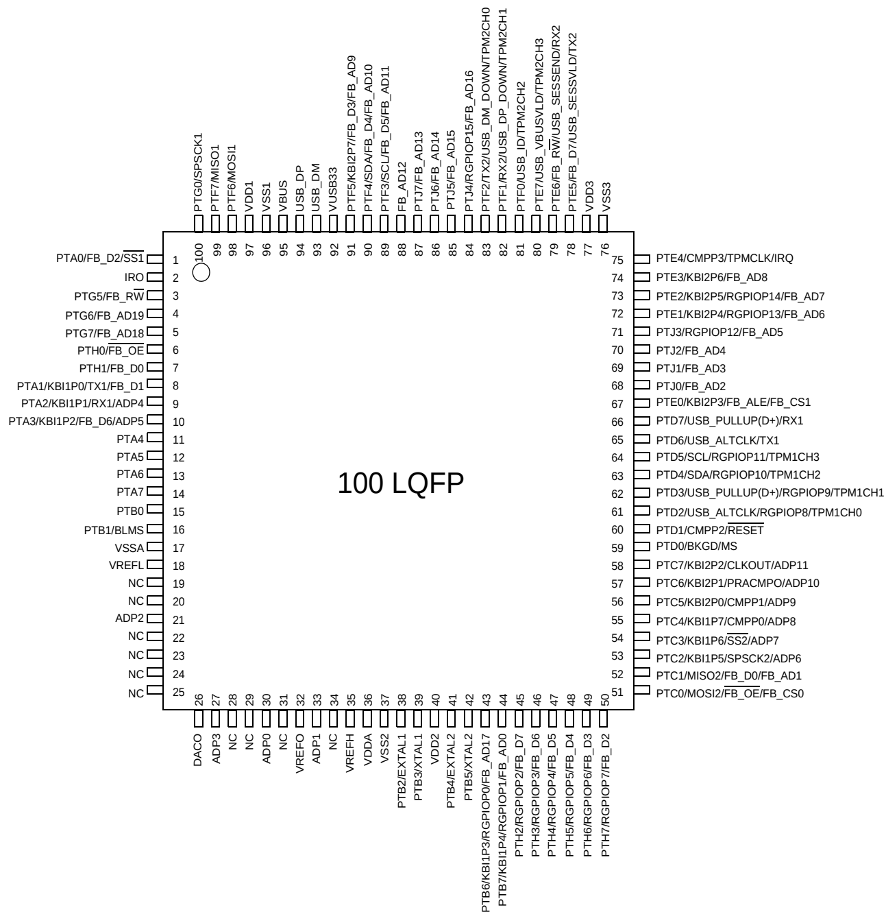
Figure 3. 100-Pin LQFP
