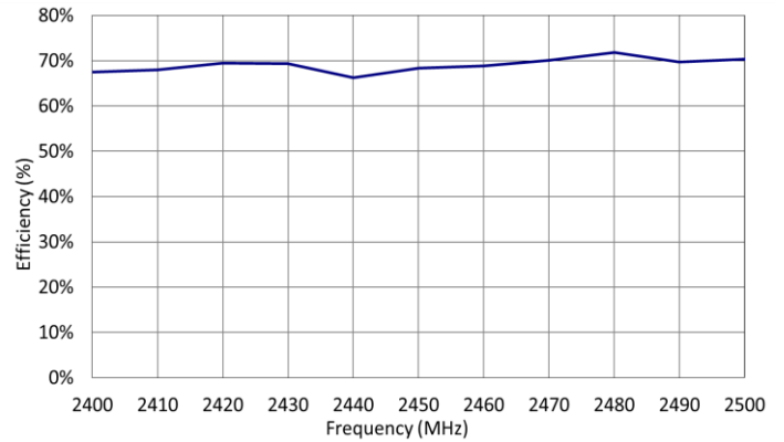
2400 MHz Efficiency
