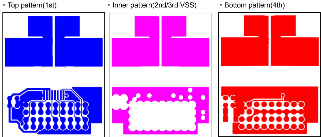
Figure 9. Board layout for measuring thermal resistance of CZ-3815
