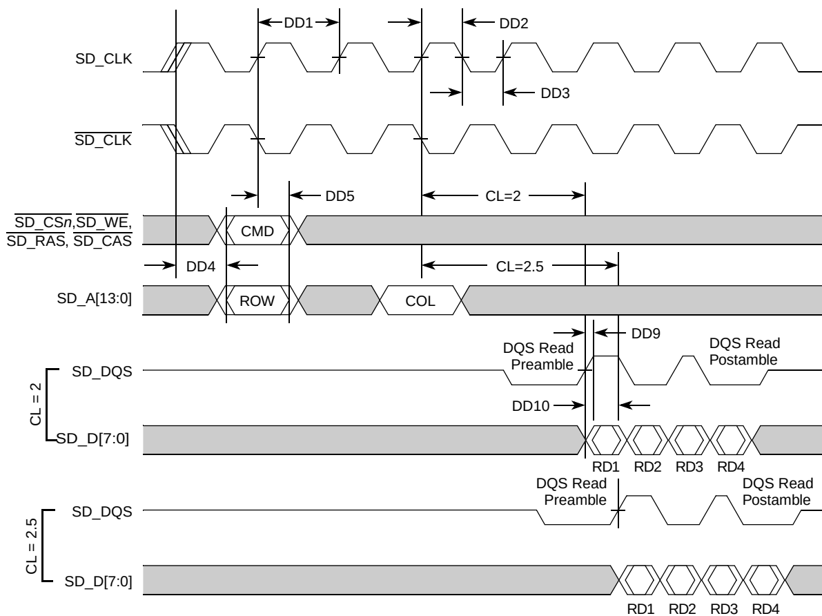
Figure 28. DDR read timing
