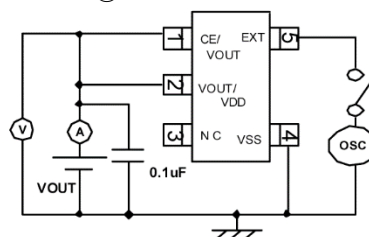
Circuit ⑦
