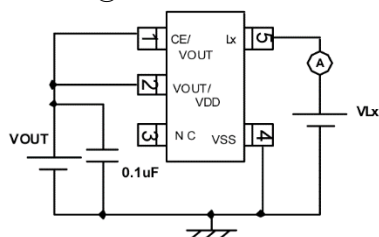
Circuit ③
