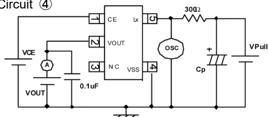
Circuit ④
