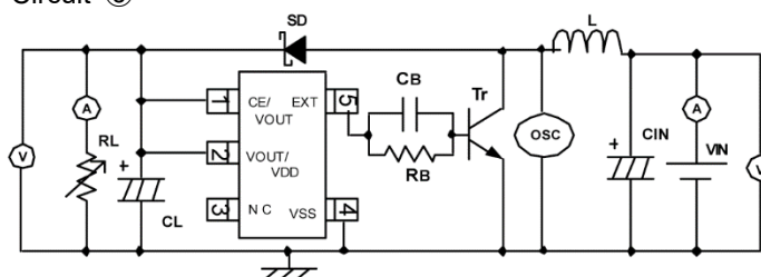
Circuit ⑥
