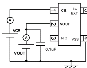
Circuit ⑥
