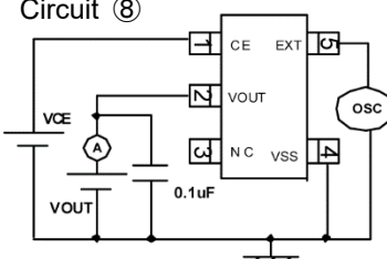
Circuit ⑧
