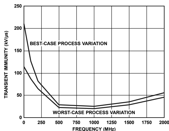
Figure 12. Transient Immunity (Sinusoidal Transients), 100°C Ambient Temperature
