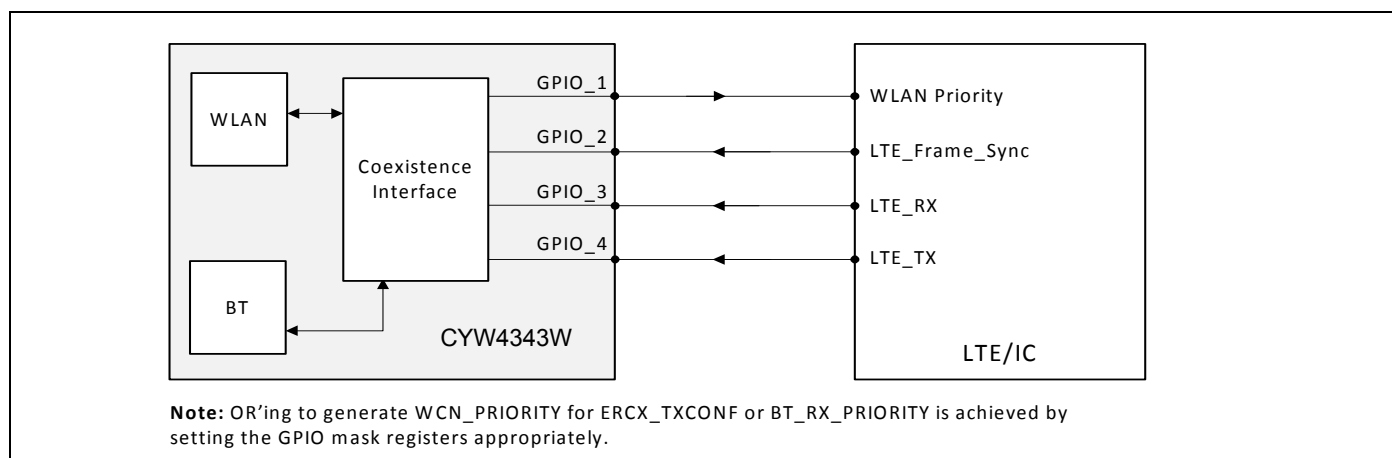
Figure 24. 4-Wire Coexistence Interface to an LTE IC
