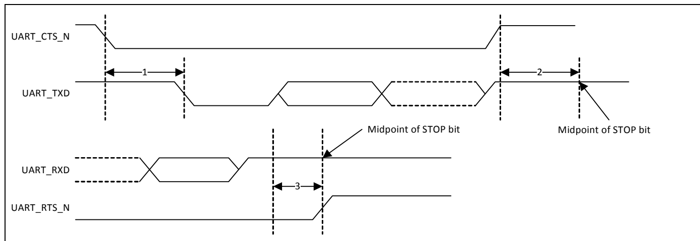
Figure 19. UART Timing
