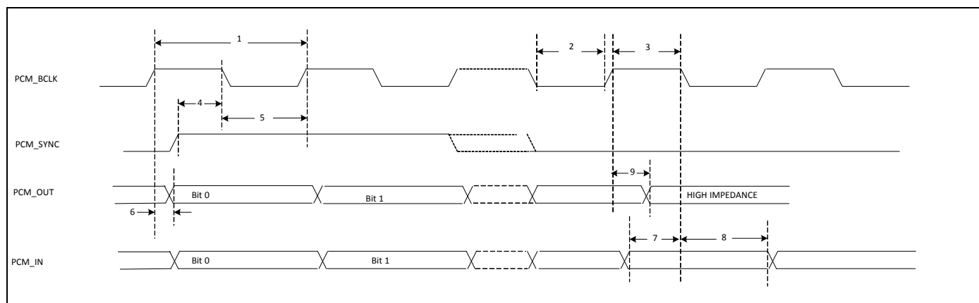
Figure 18. PCM Timing Diagram (Long Frame Sync, Slave Mode)
