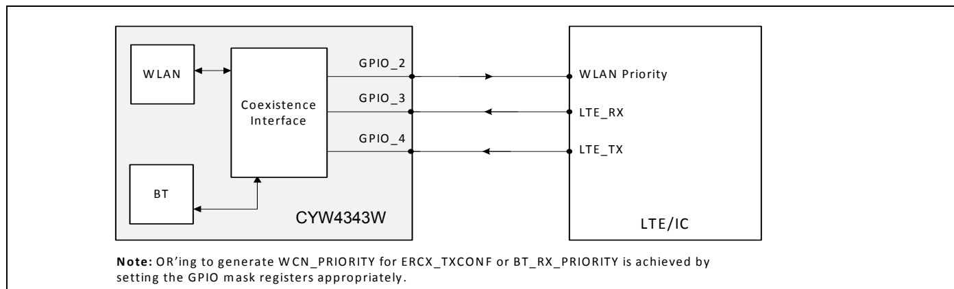
Figure 24. 4-Wire Coexistence Interface to an LTE IC
