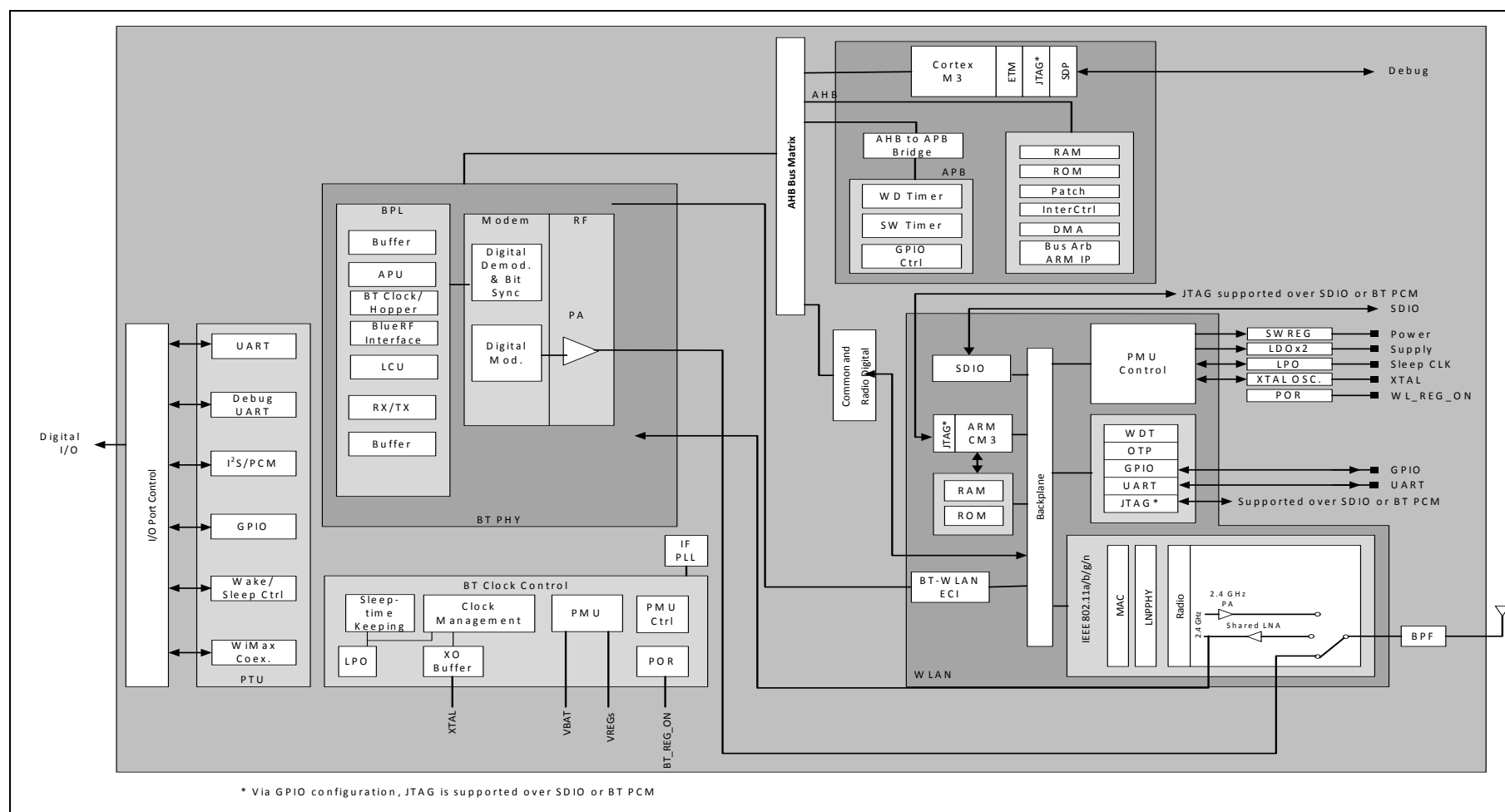
Figure 2. CYW4343W Block Diagram
