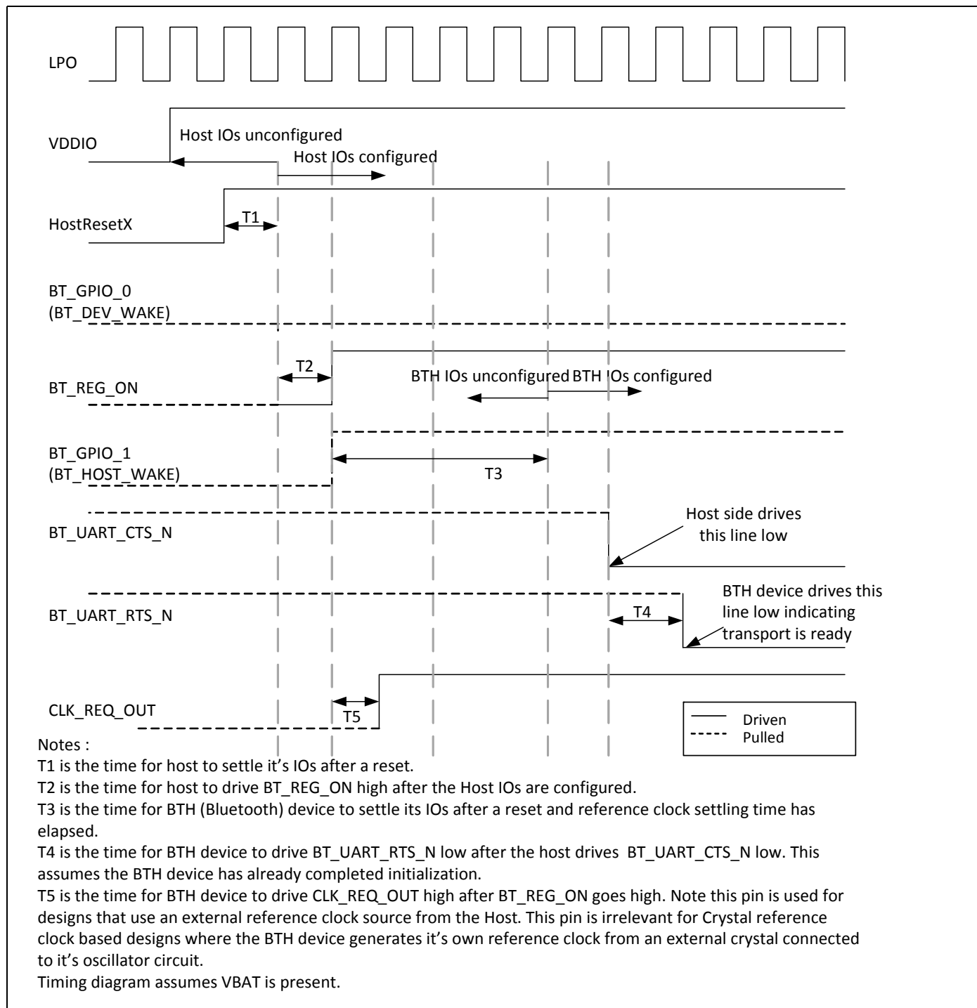
Figure 12. Startup Signaling Sequence
