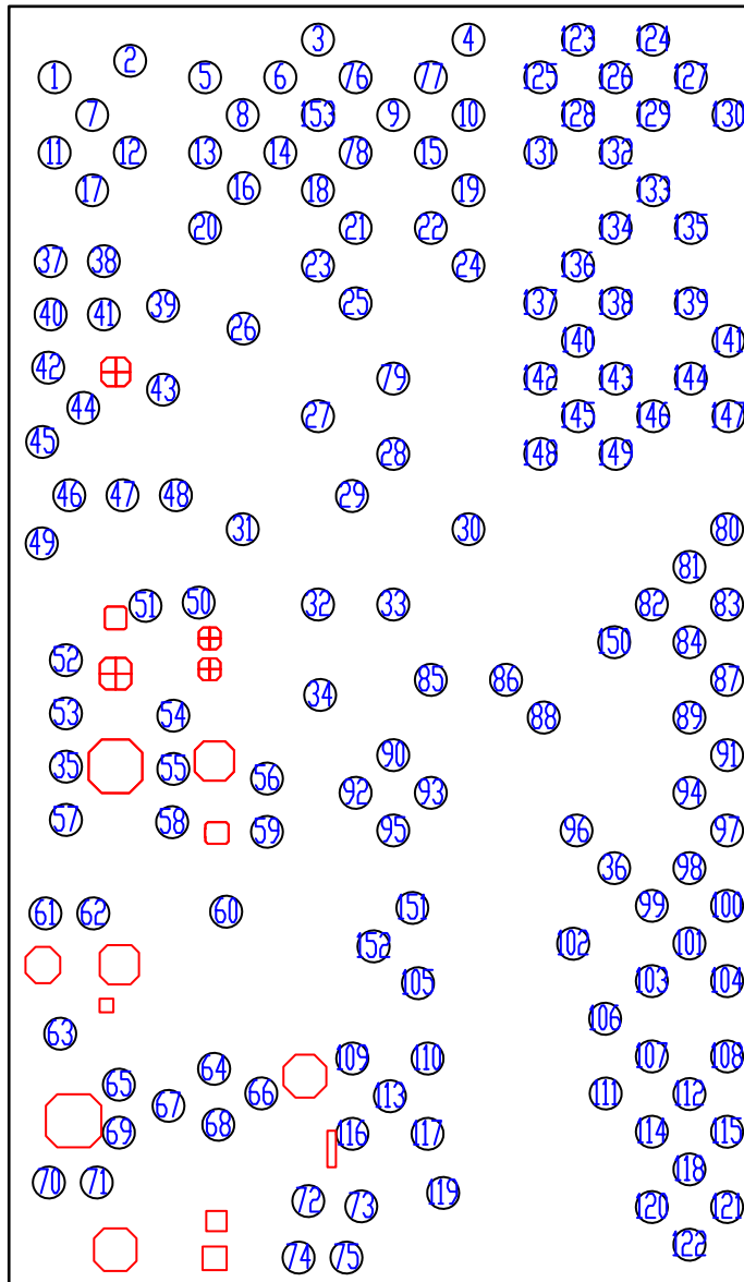
Figure 27. 153-Bump WLCSP (Top View)
