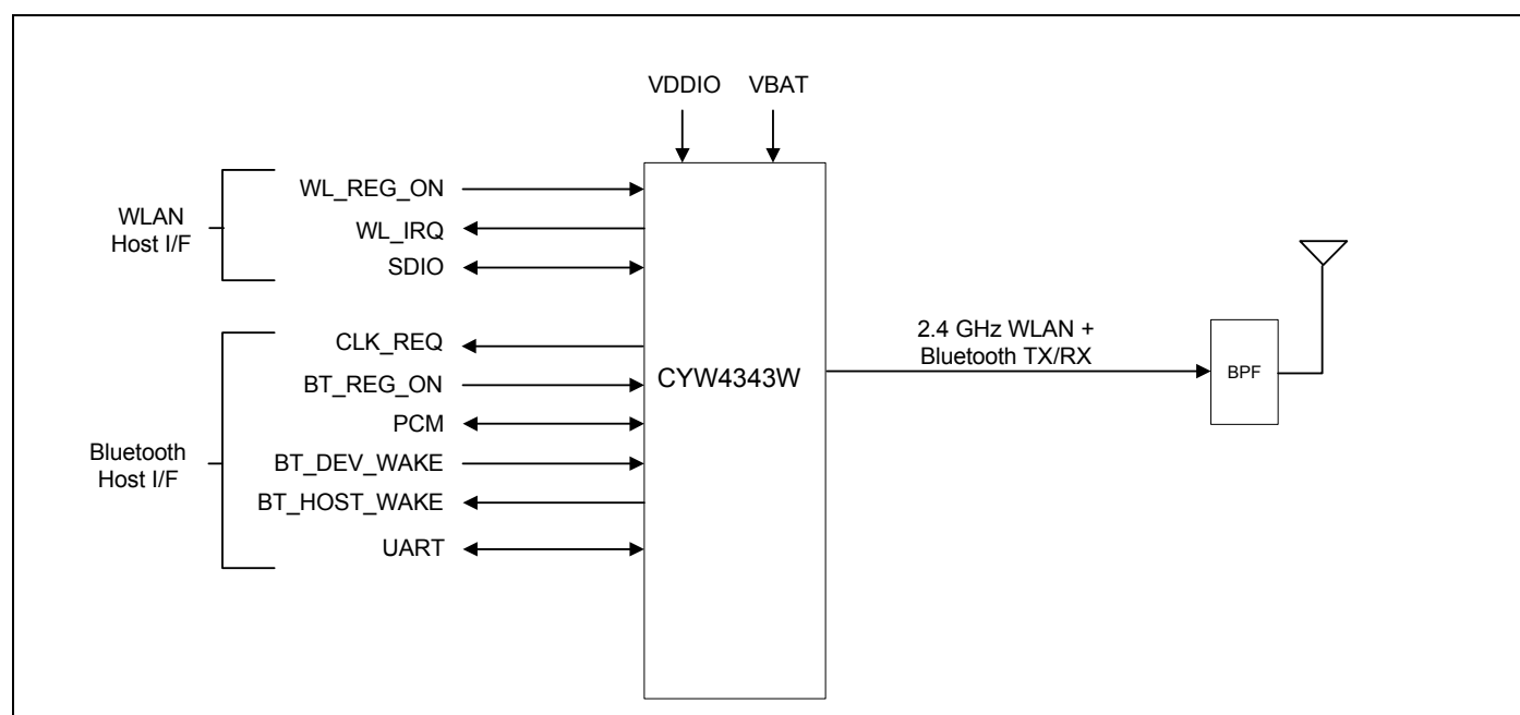
Figure 1. CYW4343W System Block Diagram
