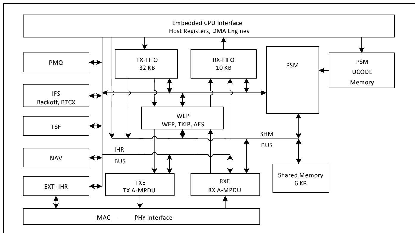
Figure 9. WLAN MAC Architecture
