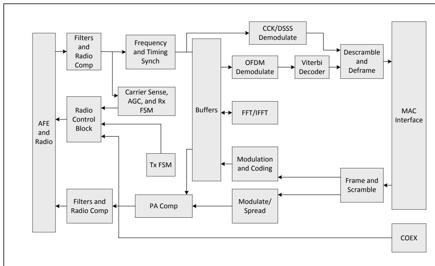
Figure 10. WLAN PHY Block Diagram
