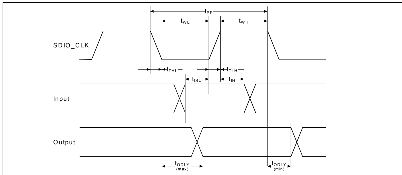
Figure 29. SDIO Bus Timing (Default Mode)
