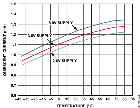
Figure 39. Quiescent Current vs. Temperature (Excludes 2\times Excitation Current)
