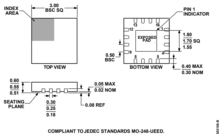
COMPLIANT TO JEDEC STANDARDS MO-248-UEED. Figure 49. 16-Lead Lead Frame Chip Scale Package [LFCSP_UQ] 3 mm × 3 mm Body, Ultra Thin Quad (CP-16-12) Dimensions shown in millimeters
