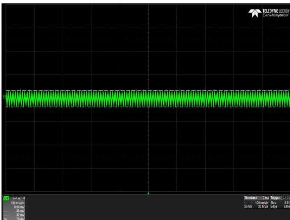
Figure 9: DS1600SPE-3 Ripple and Noise Measurement – Vin = 90Vac Full Load: Io = 63.2A, Isb = 3.5A Ch 4: Vo
