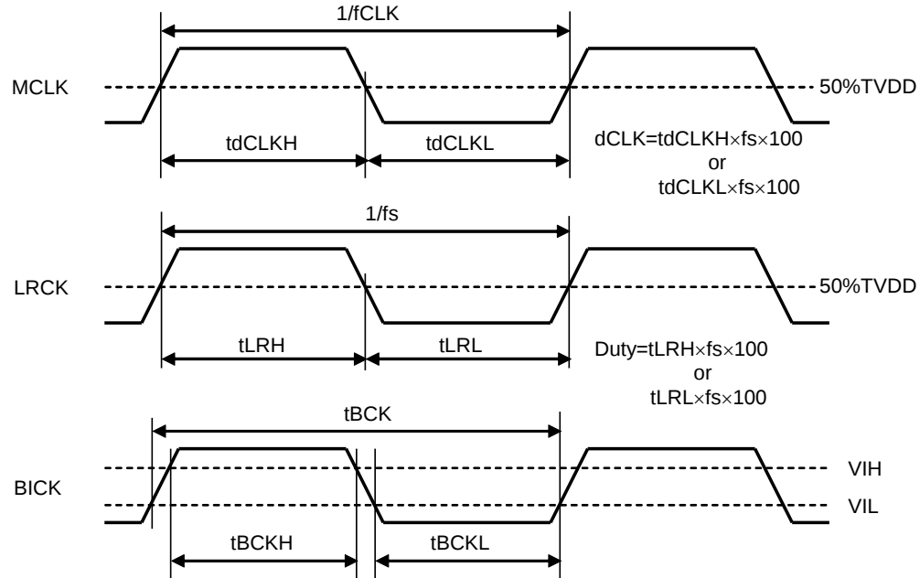
Figure 17. Clock Timing (Slave Mode)
