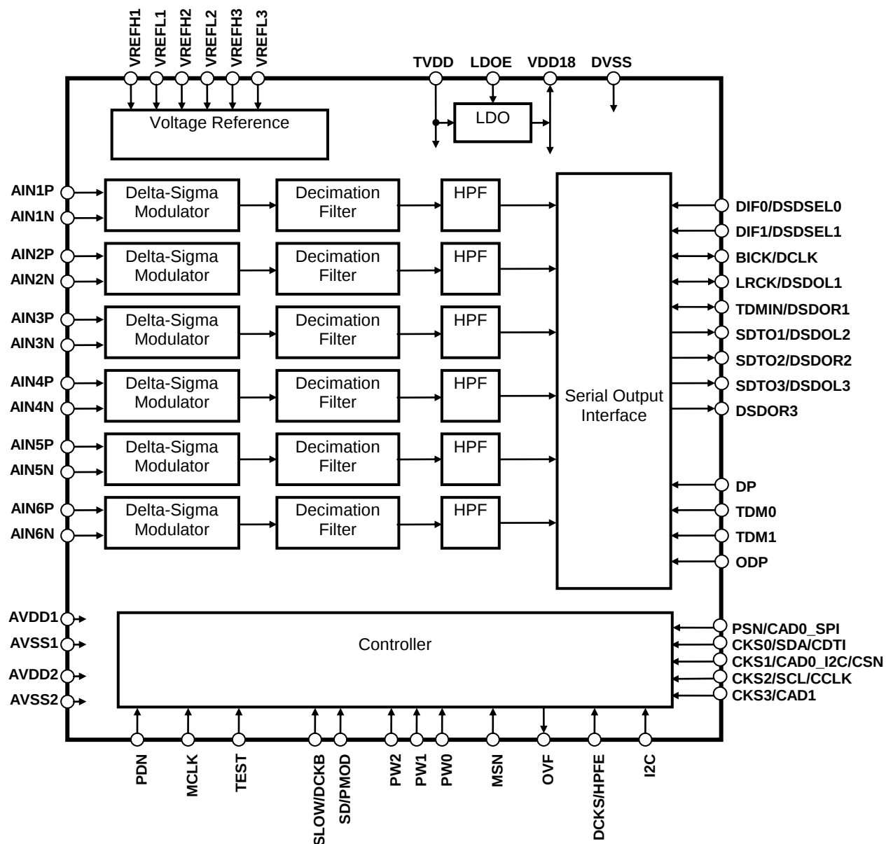
Figure 1. Block Diagram
