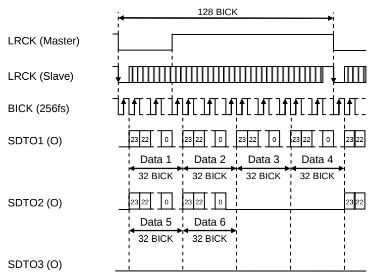
Figure 43. Mode 25/29 Timing (TDM128 Mode, I 2 S Compatible)
