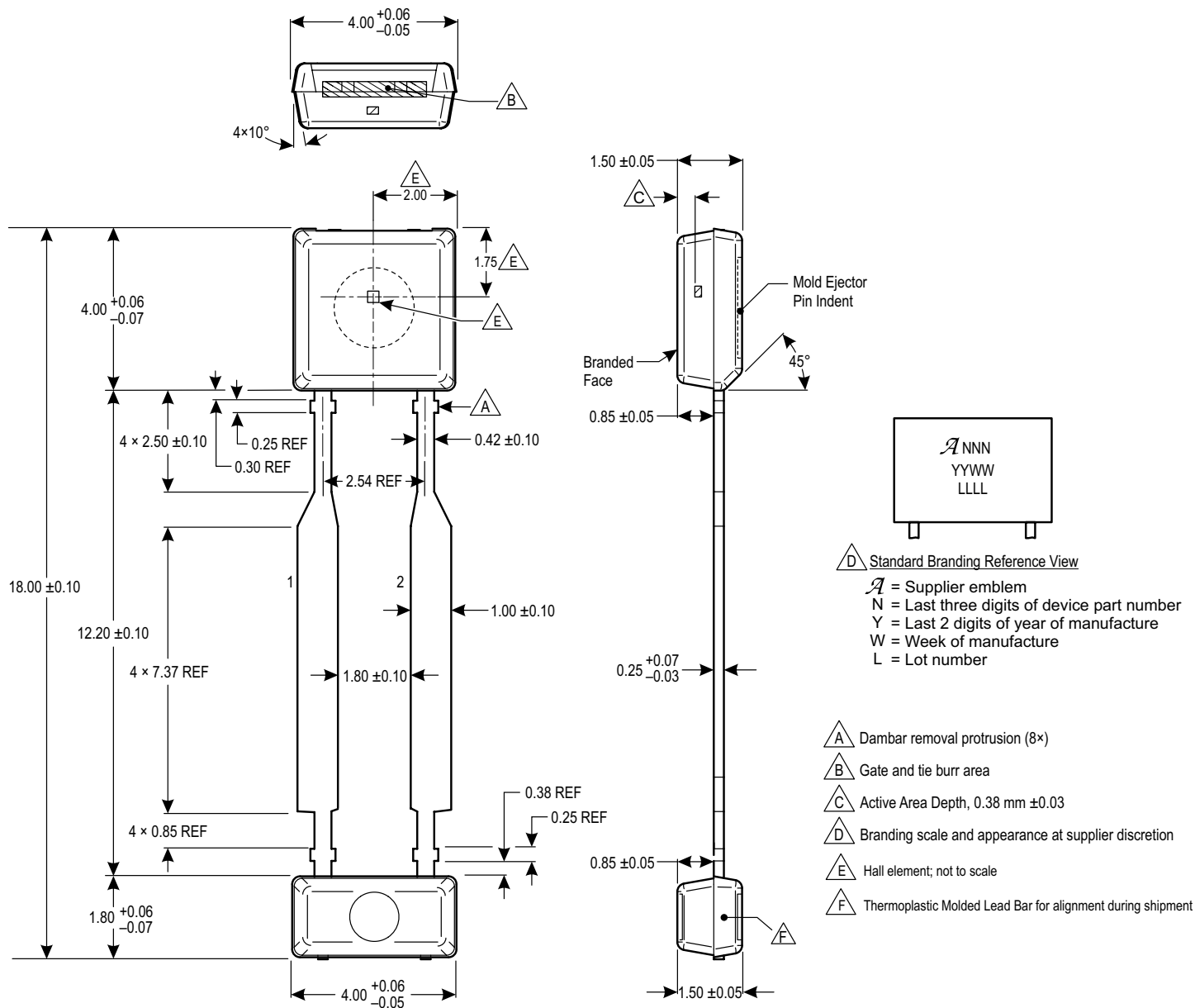
Package UB, 2-Pin SIP
