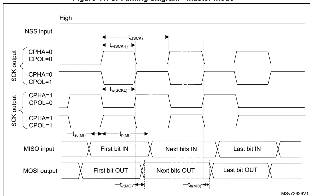
Figure 41. SPI timing diagram - master mode (1)
