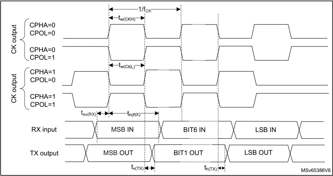
Figure 53. USART timing diagram in SPI master mode
