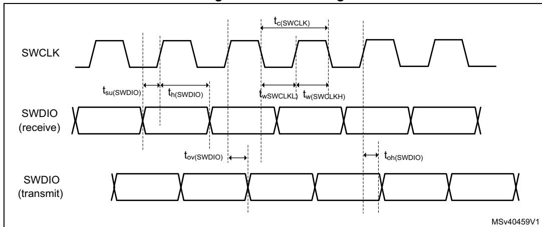
Figure 56. SWD timing
