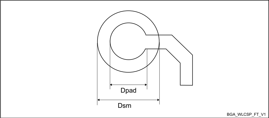
Figure 60. TFBGA289 - Recommended footprint
