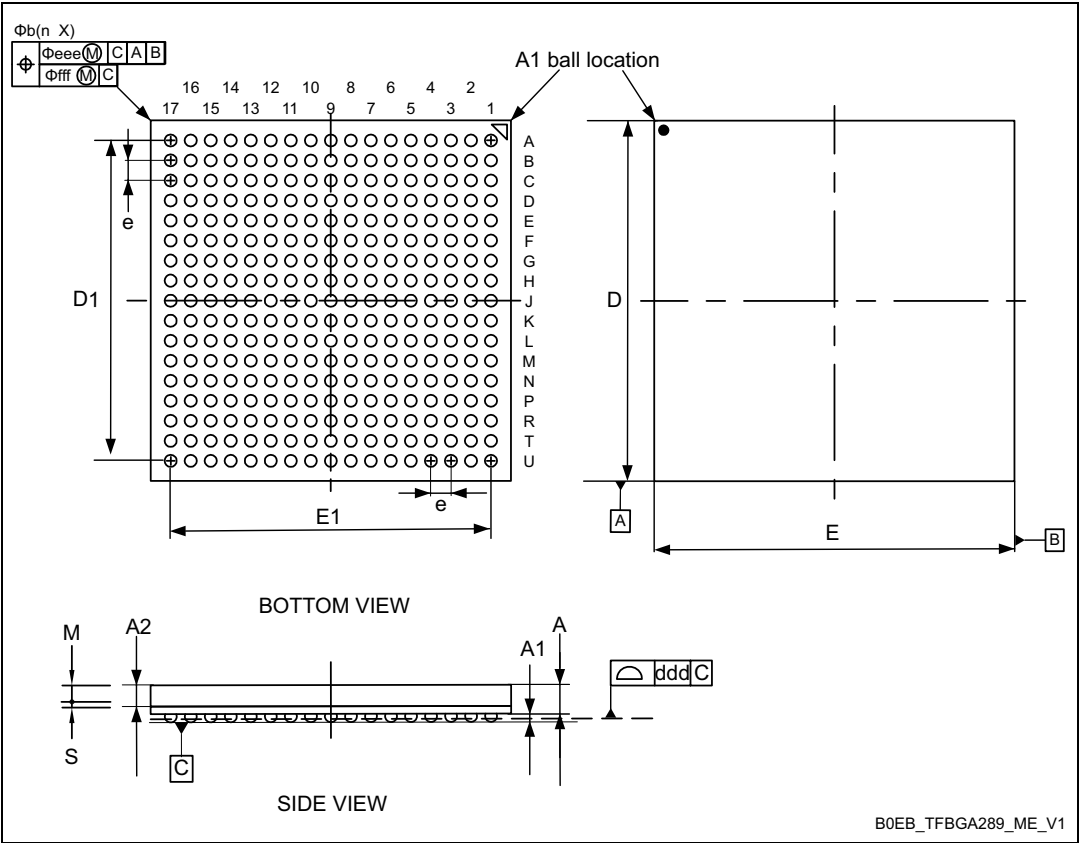
Figure 59. TFBGA289 - Outline
