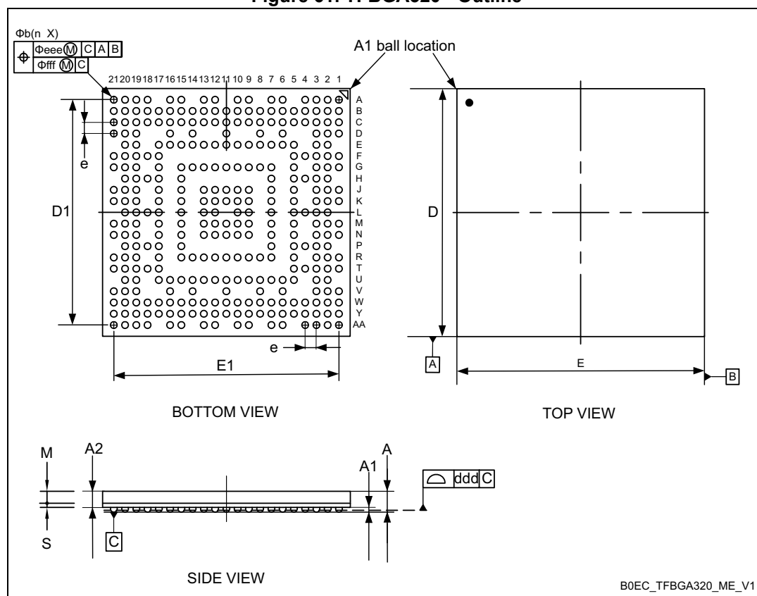
Figure 61. TFBGA320 - Outline
