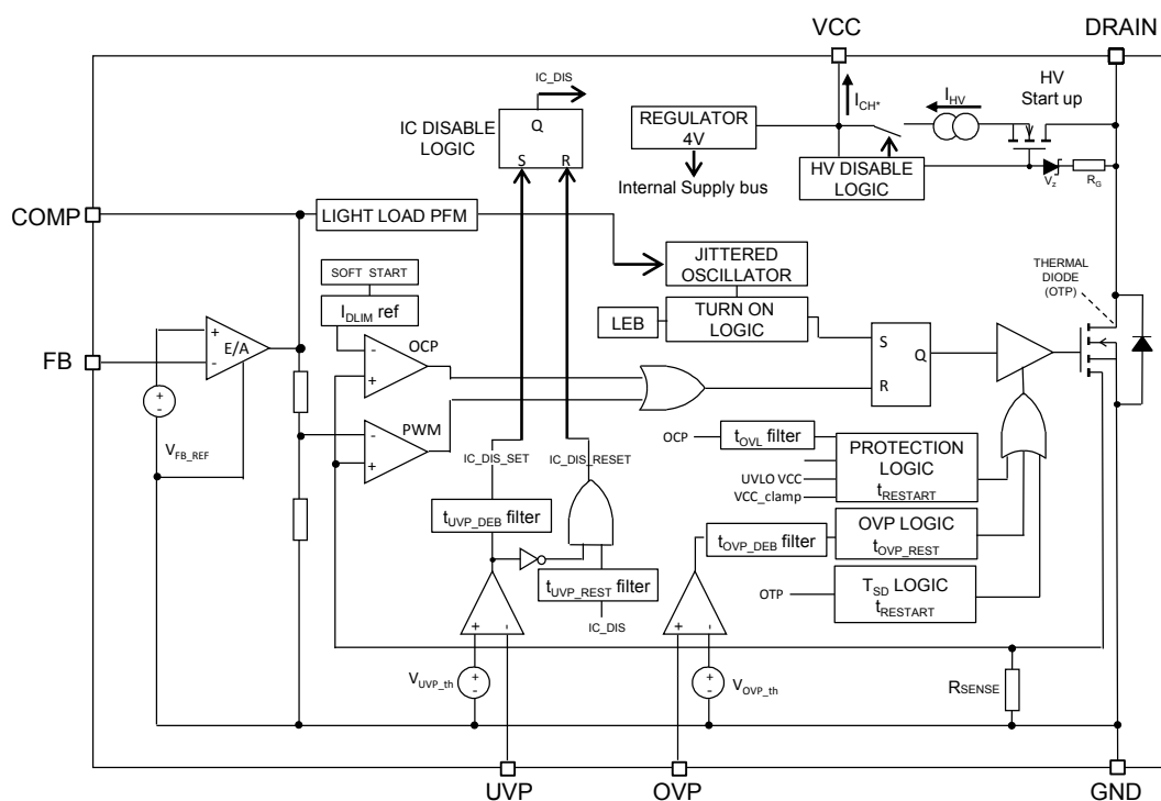
Figure 23. Block diagram
