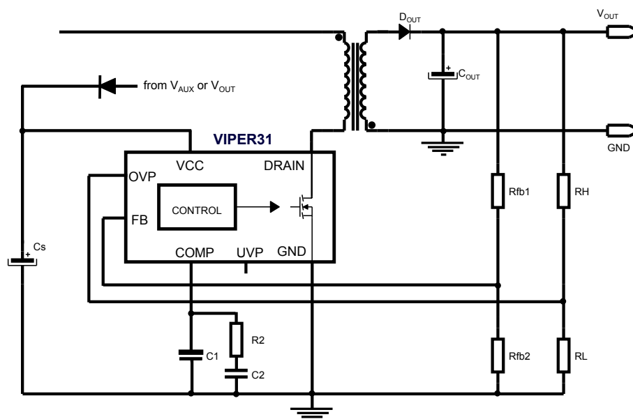
Figure 34. Connection for output overvoltage protection (non-iso topologies)
