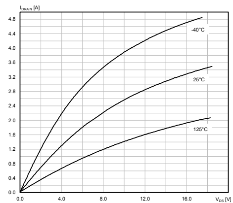
Figure 20. Output characteristic
