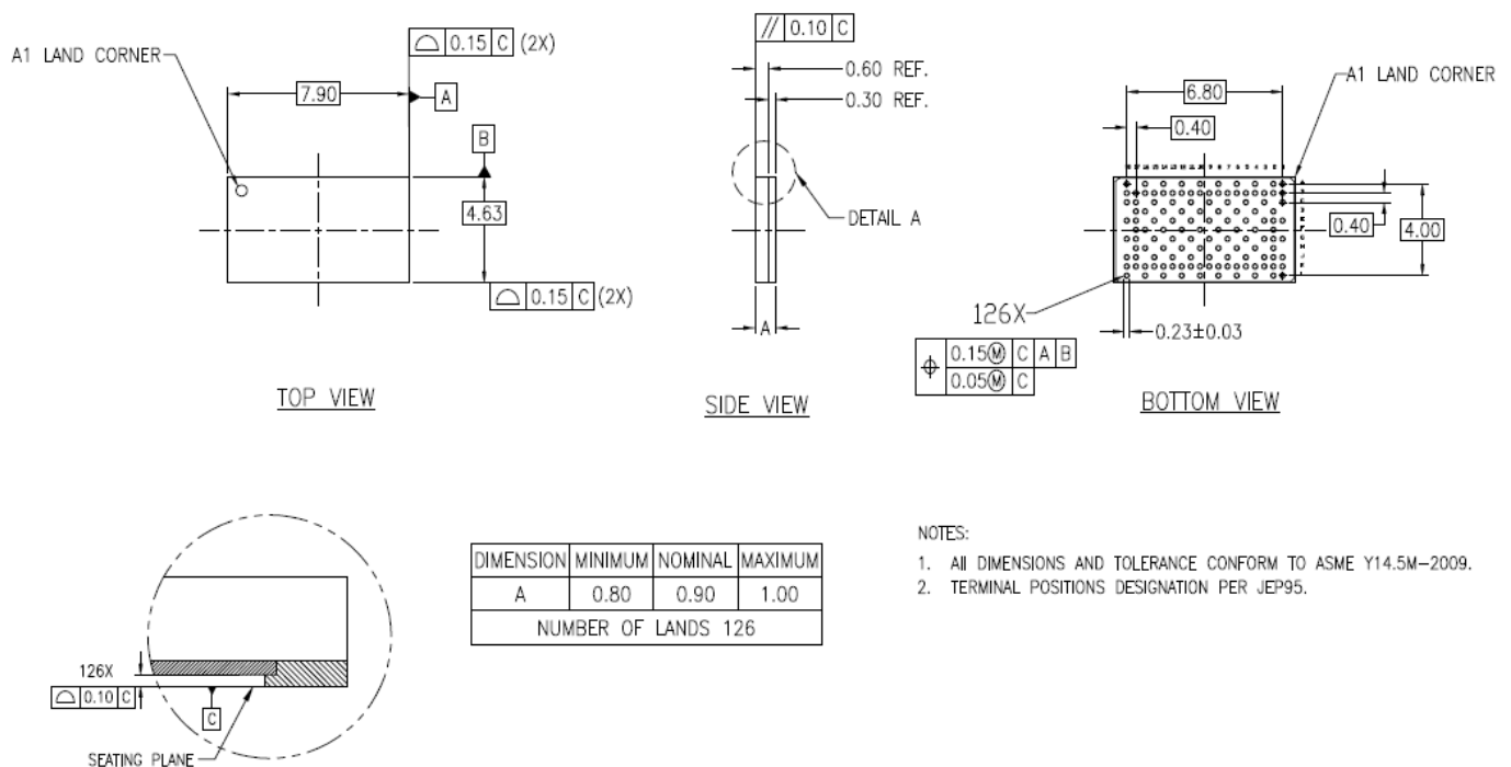
Figure 22. Module Dimensions
