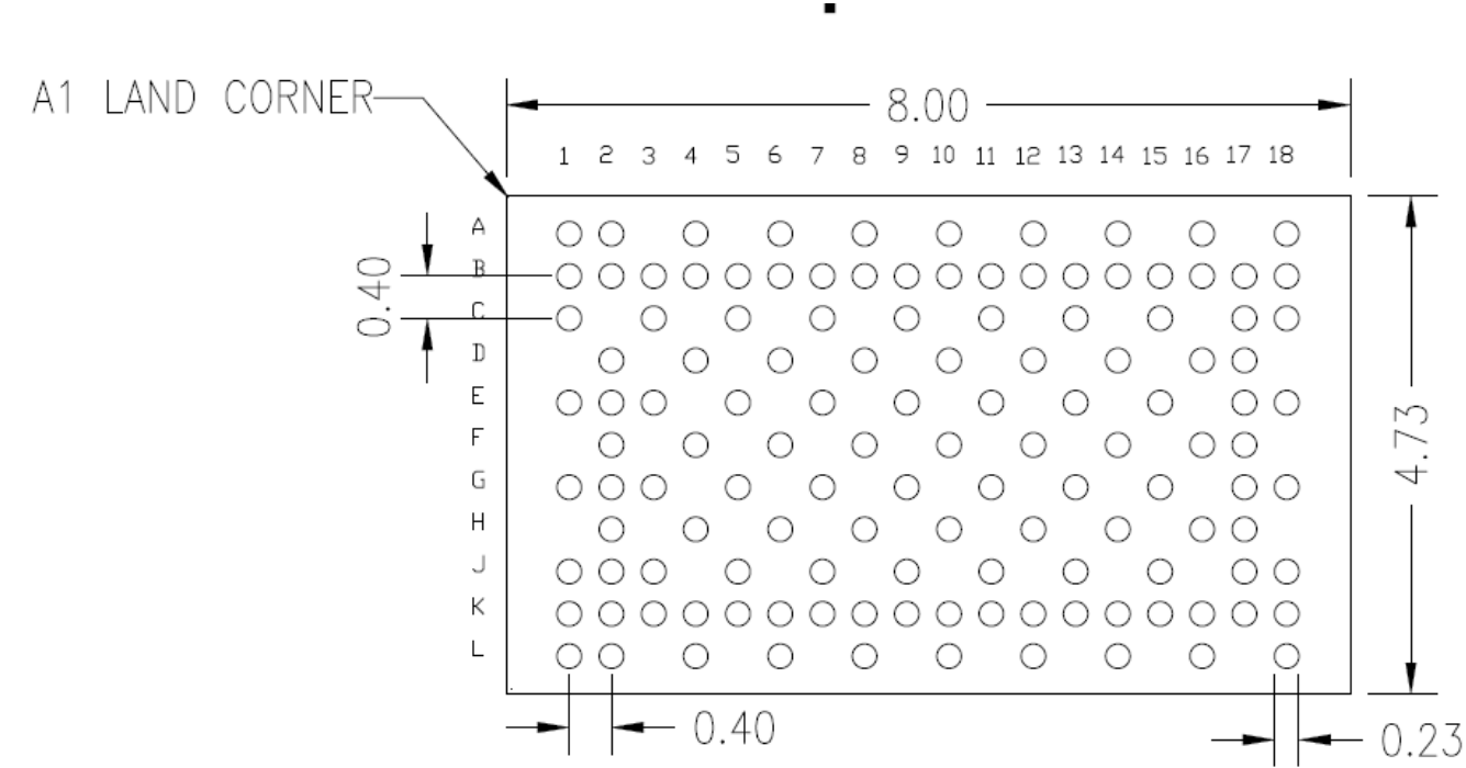
Figure 23. PCB Landing Pattern
