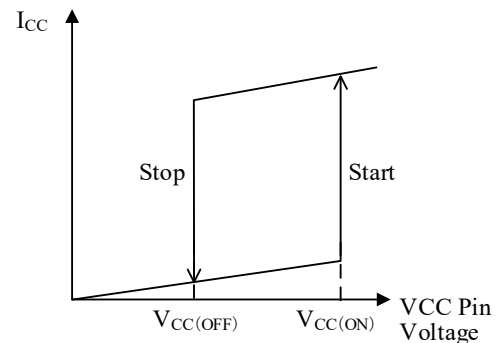
Figure 9-15. V_{\text{CC}} vs. I_{\text{CC}}
