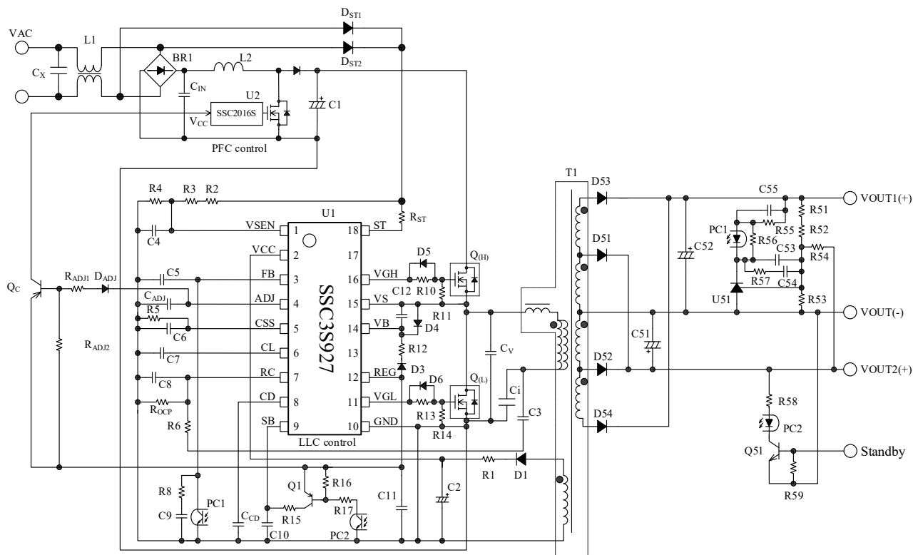
Figure 6-1. Typical Application
