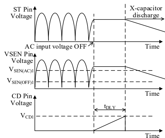
Figure 9-36. Operational Waveform of X-capacitor Discharge Function
