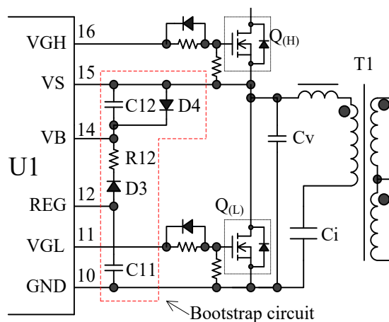
Figure 9-19. Bootstrap Circuit
