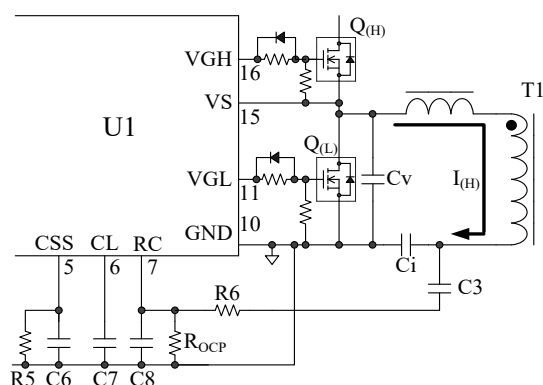
Figure 9-42. RC Pin Peripheral Circuit
