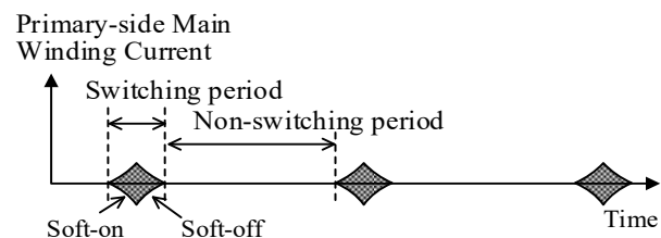
Figure 9-21. Standby Waveform
