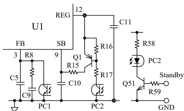
Figure 9-22. Standby Mode Switching Circuit
