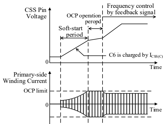
Figure 9-17. Soft-start Operation
