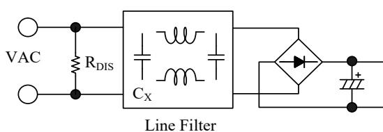
Figure 9-34. Typical Line Filter Circuit
