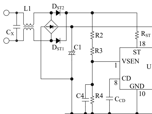
Figure 9-40. VSEN Pin Peripheral Circuit
