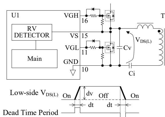
Figure 9-28. VS Pin and Dead Time Period
