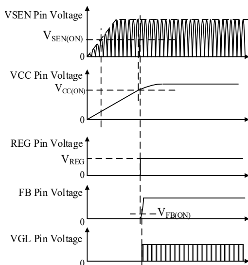
Figure 9-14. The Startup Operation When PFC On/Off Function is Disabled
