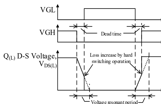
Figure 9-27. ZVS Failure Operation Waveform
