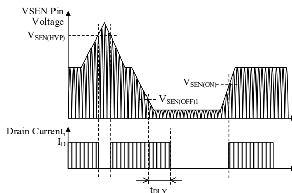
Figure 9-41. Input Voltage Detection Function Operational Waveforms
