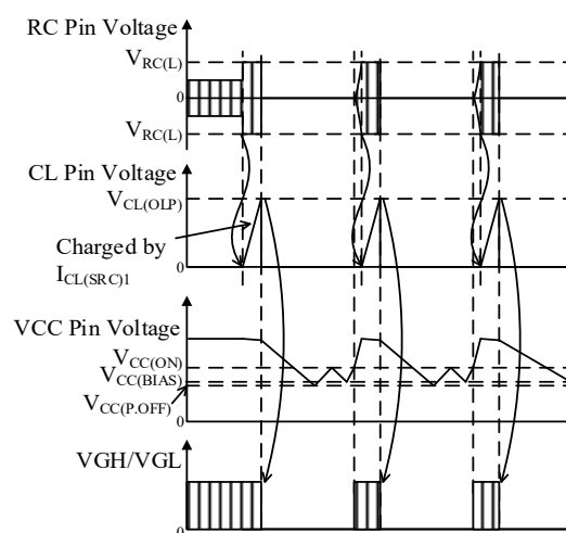
Figure 9-43. OLP Waveform
