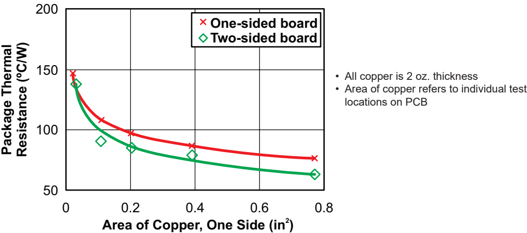
Figure 2: Thermal Resistance ( R_{\theta JA} ) versus Copper Area on Printed Circuit Board (PCB)
