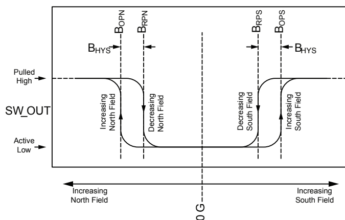
Figure 4: Hall Switch Output ( \overline{SO} ) State versus Magnetic Field (POL = GND)
