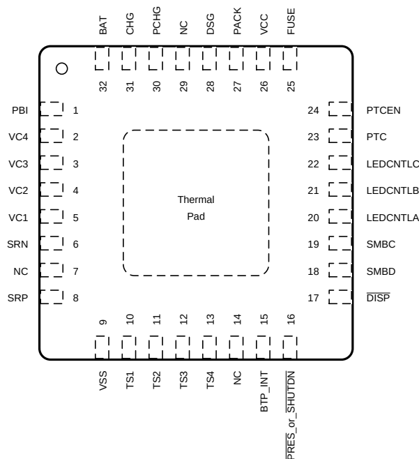
Pin Functions
