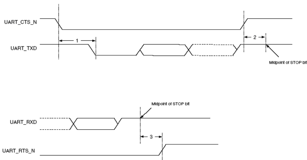
Figure 12. UART Timing
