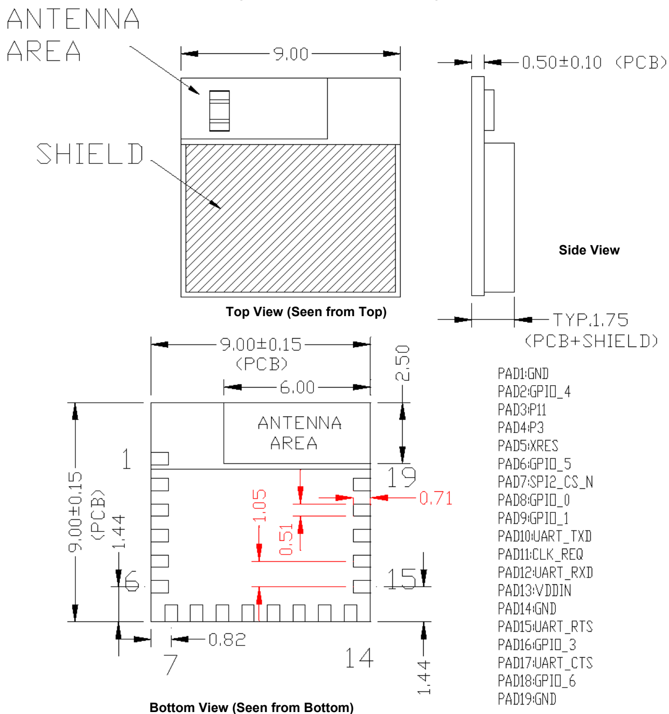
Figure 2. Module Mechanical Drawing [2]
