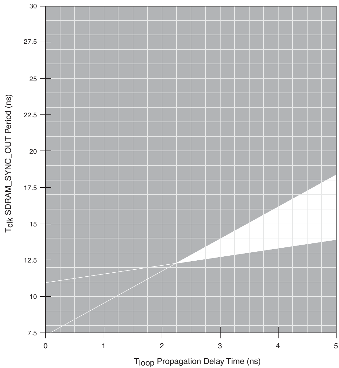
Figure 2-5. DLL Locking Range Loop Delay Versus Frequency of Operation for DLL_Extend = 1 and Max Tap Delay
