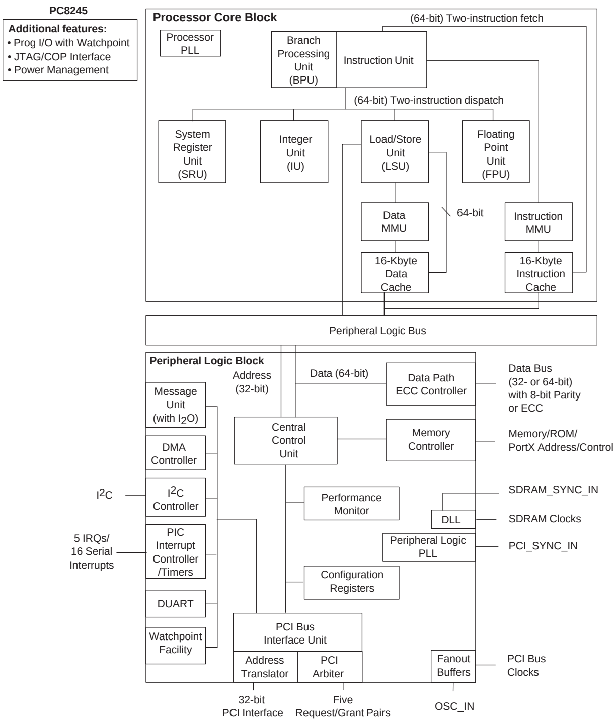
Figure 1-1. Block Diagram
