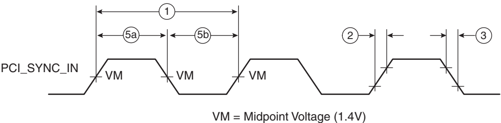
Figure 2-1. PCI\_SYNC\_IN Input Clock Timing Diagram
