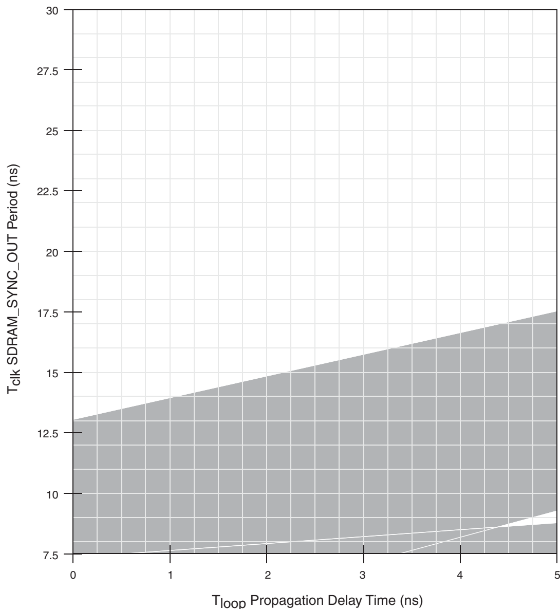
Figure 2-2. DLL Locking Range Loop Delay Versus Frequency of Operation for DLL_Extend = 0 and Normal Tap Delay
