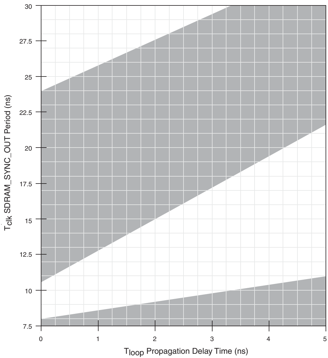
Figure 2-3. DLL Locking Range Loop Delay Versus Frequency of Operation for DLL_Extend = 1 and Normal Tap Delay
