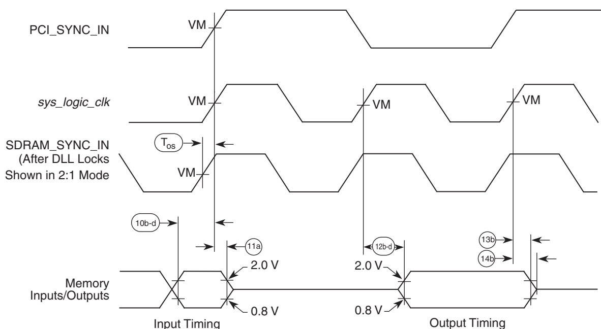
Figure 2-6. Input – Output Timing Diagram Referenced to SDRAM_SYNC_IN
