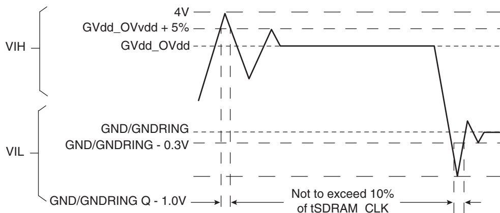
Figure 1-3. Overshoot/Undershoot Voltage
