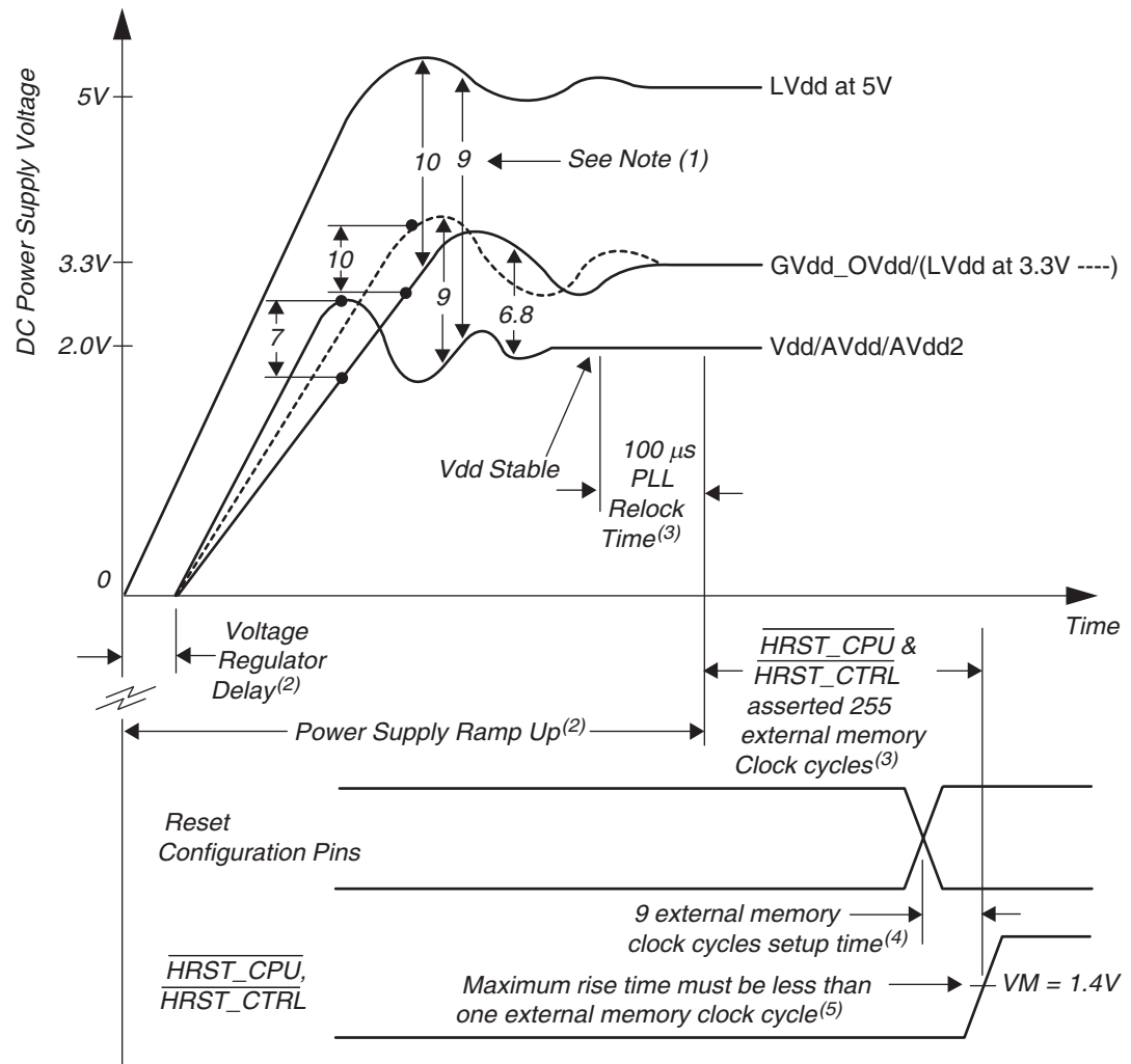
Figure 1-2. Supply Voltage Sequencing and Separation Cautions
