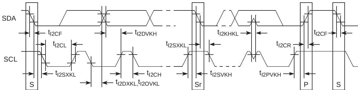
Figure 2-12. I 2 C Bus AC Timing Diagram
