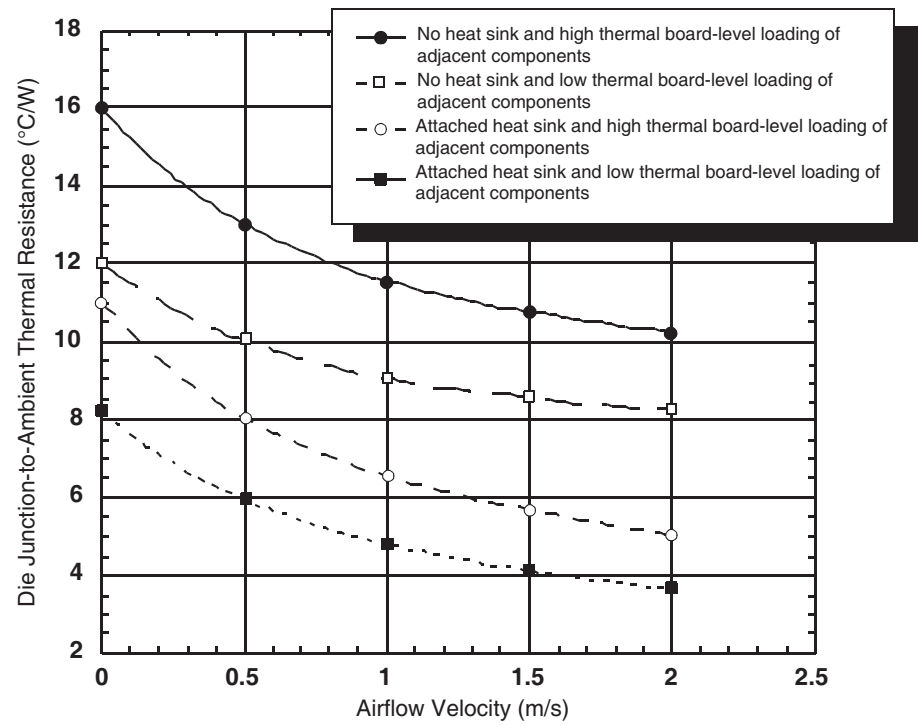
Figure 1-7. Die Junction-to-Ambient Resistance
