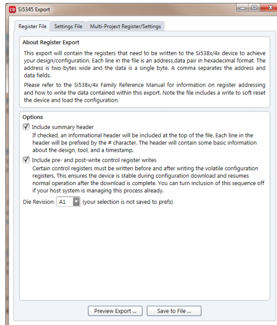
Figure 27. Export Settings
