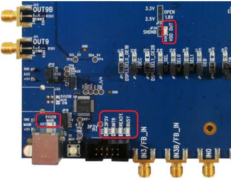
Figure 3. Status LEDs
