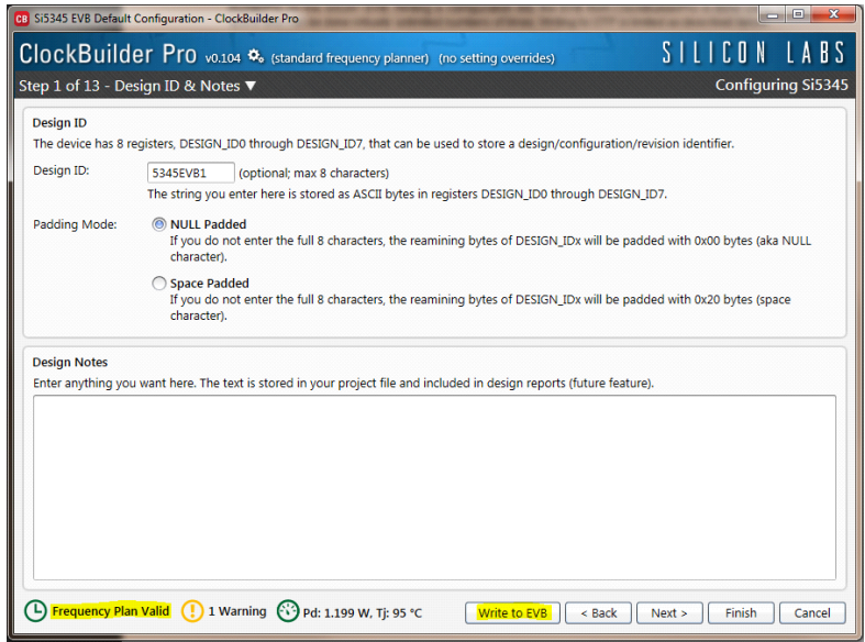
Figure 21. Design Wizard
