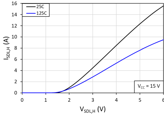
Fig. 7. Source-to-drain reverse conduction voltage ( I_{SDL,H} ) vs. drain-to-source voltage ( V_{DSL,H} ) at T = 25\text{ }^\circ\text{C} and 125\text{ }^\circ\text{C}
