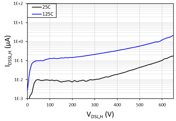
Fig. 8. Drain-to-source leakage current ( I_{DSSL,H} ) vs. drain-to-source voltage ( V_{DSL,H} ) at T = 25\text{ }^\circ\text{C} and 125\text{ }^\circ\text{C}
