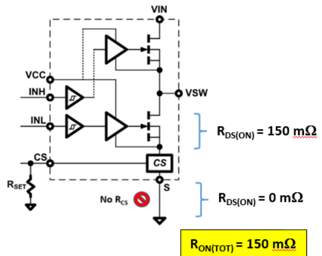
Fig. 30. External current sensing resistor vs. GaNSense™ Technology
