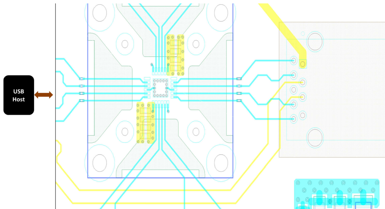
Figure 8-3. Example Layout
