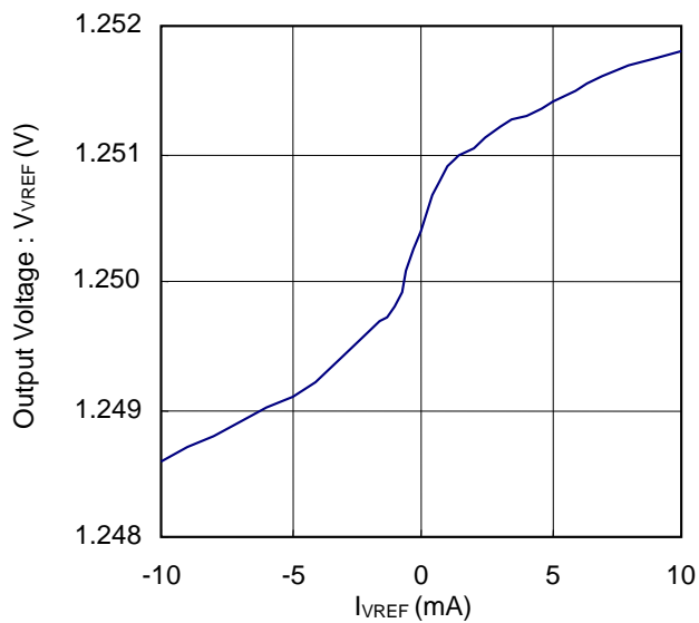
Figure 9. Output Voltage vs I_{VREF} (DDR1)
