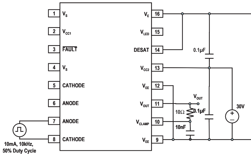
Figure 29. t_{PLH} , t_{PHL} , t_r , t_f test circuit
