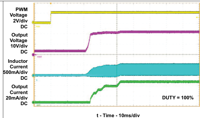
Figure 2. Start-Up Waveform
