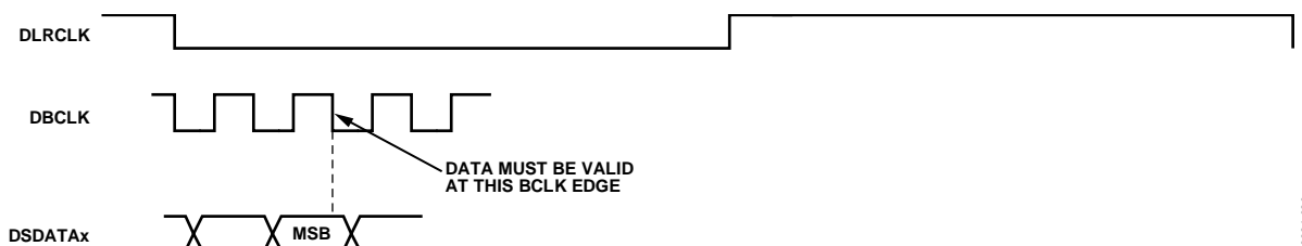
Figure 20. Pipeline Mode in DAC Serial Data Transmission (Applicable in Stereo and TDM Useful for High Frequency TDM Transmission)
