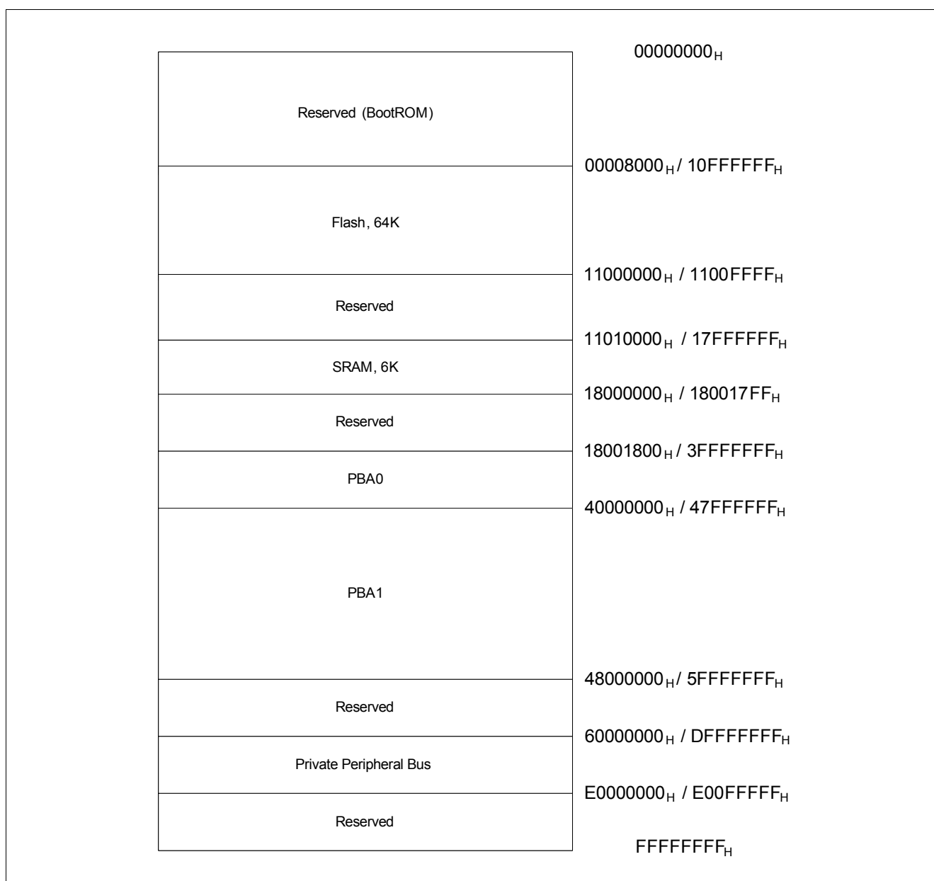
Figure 14 TLE9867QXA20 Memory Map
